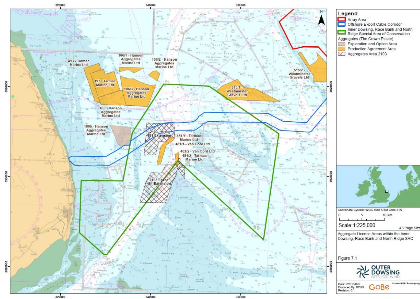
Figure 7.1 Aggregate licence areas within the IDRBNR SAC
