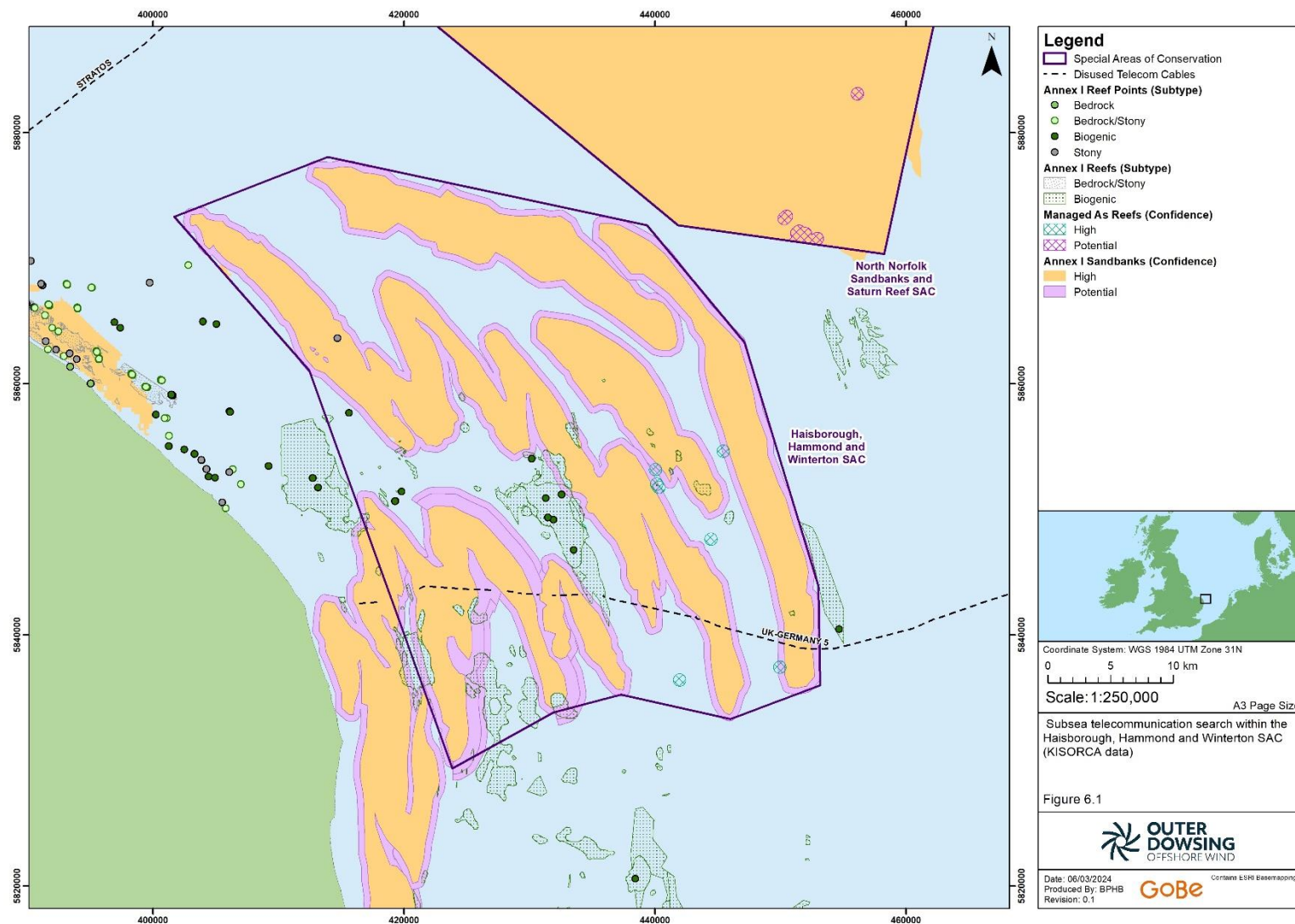
Figure 6.1 Subsea telecommunication search within the HHW SAC (KISORCA data).
